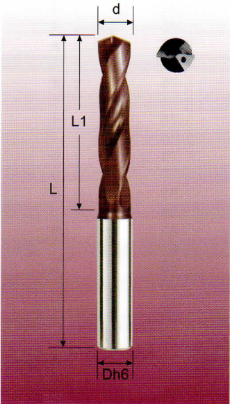
CUTTING EFFECTED LENGTH = 5xD
