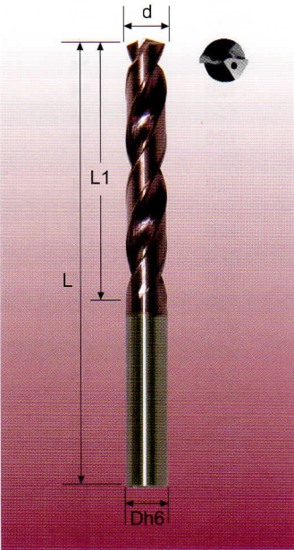
CUTTING EFFECTED LENGTH = 7xD
